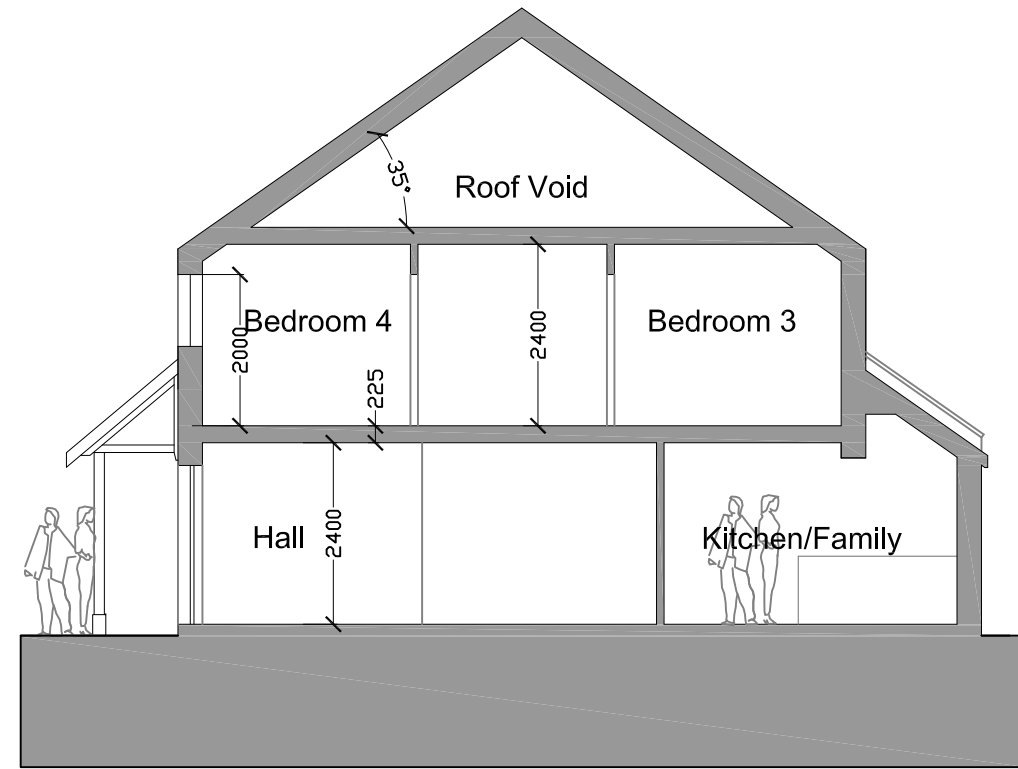
Proposed Section Through
