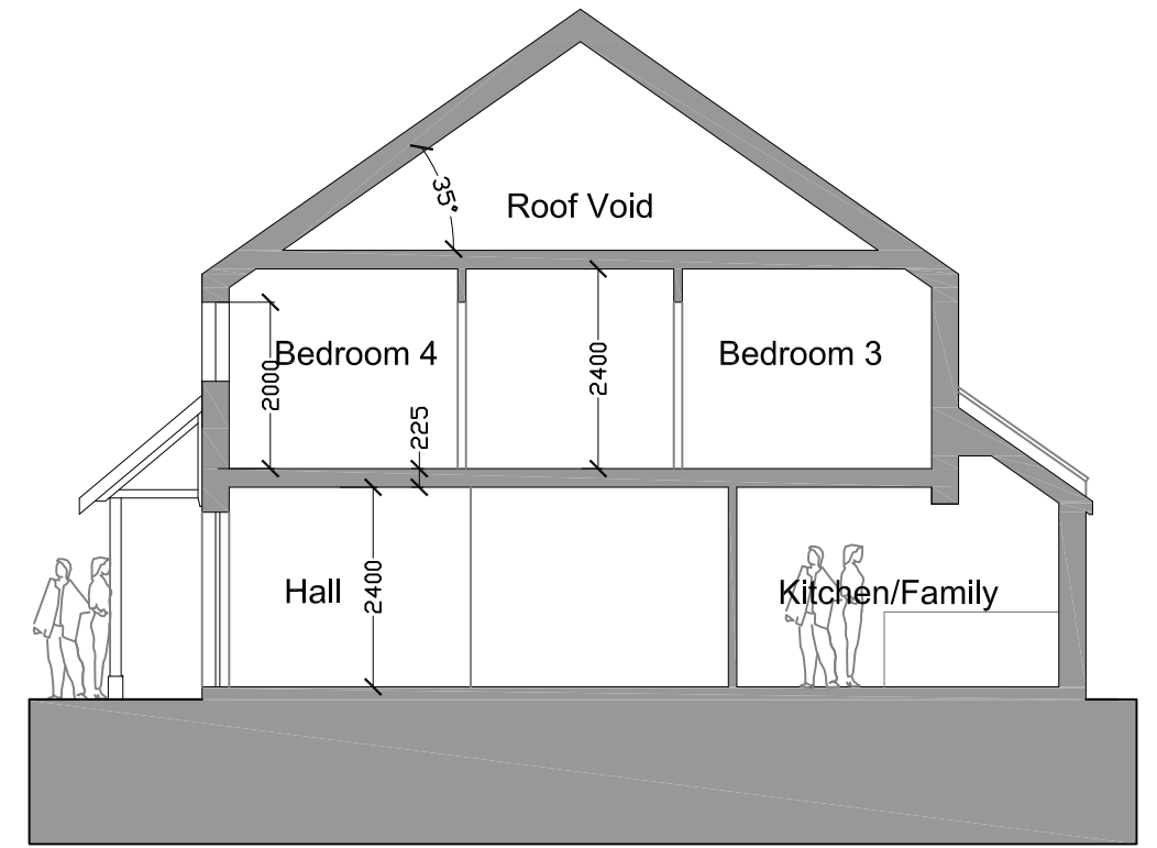
Proposed Section Through
